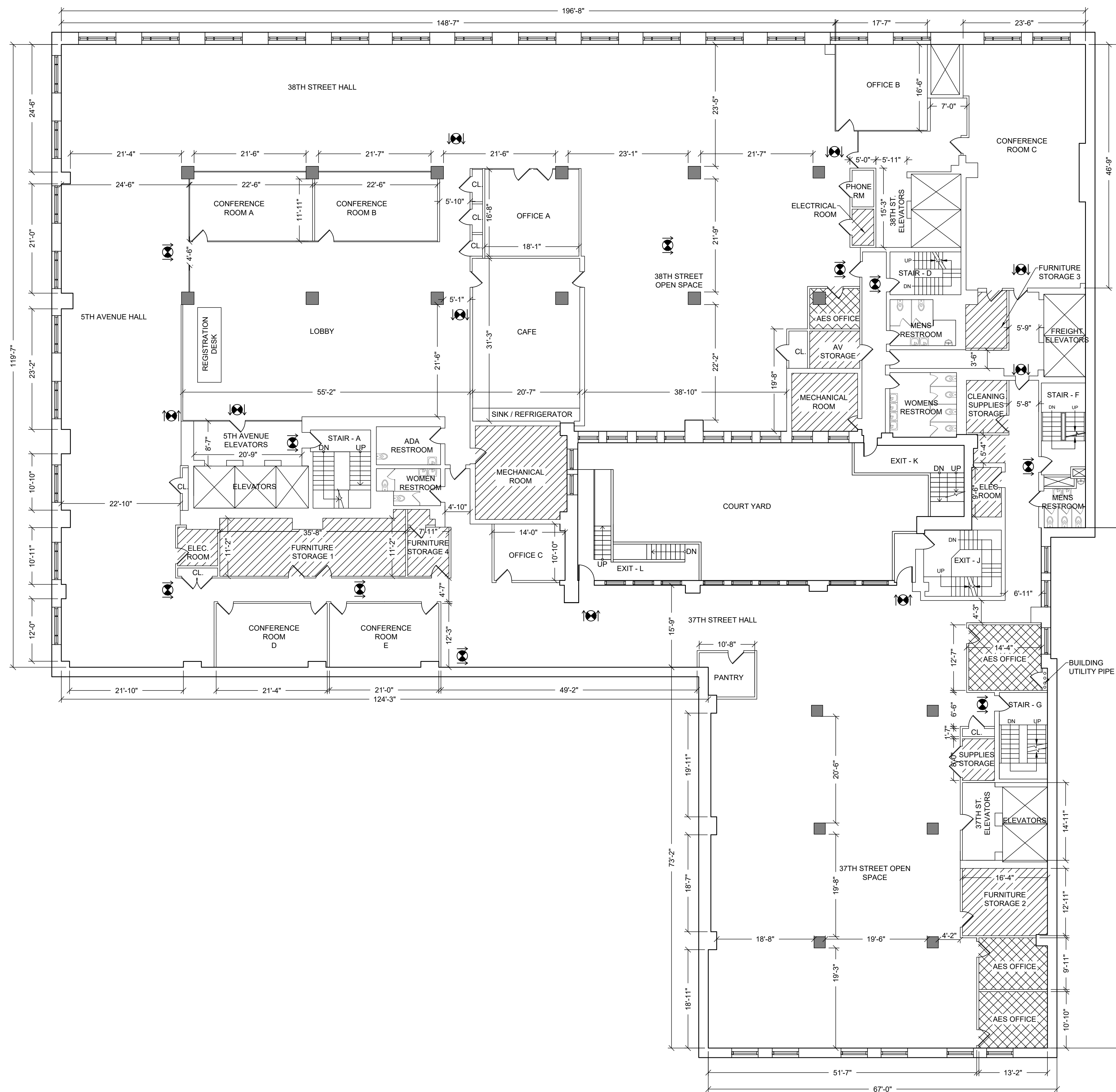
1 7TH FLOOR PLAN SCALE: 3/32" = 1' - 0"
